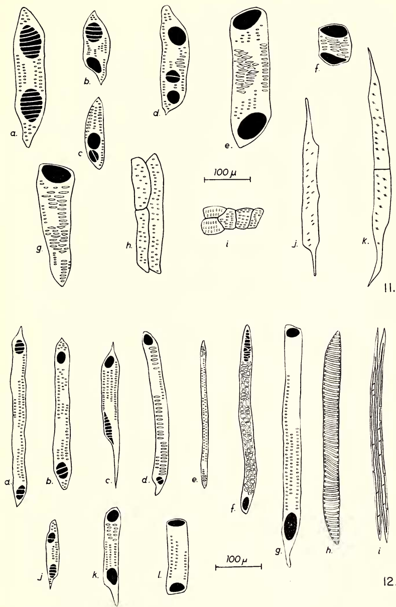
FIGS. 11-12. Tracheary elements of Laurus nobilis : 11, root wood; 12, stem wood. (Explanation in text).
